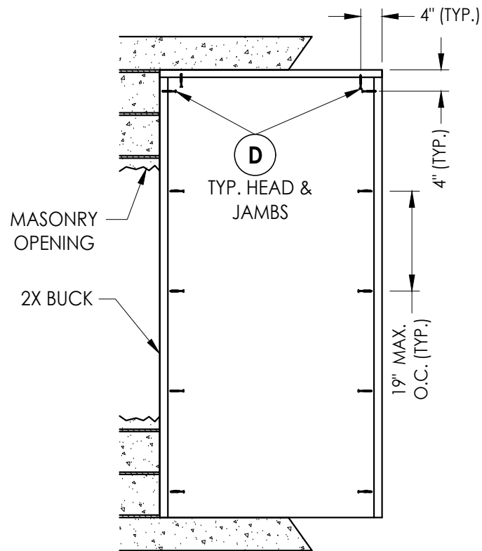
BUCK ANCHORING
