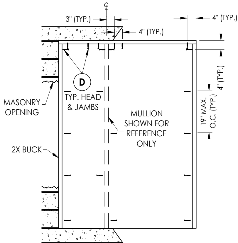
BUCK ANCHORING
